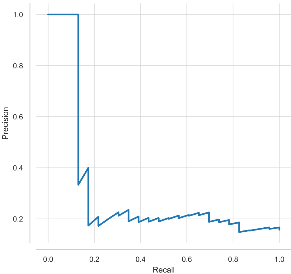
Precision-Recall Curve - SVC
